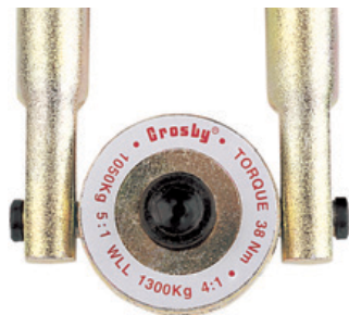
HR-125M Swivel Hoist Ring
